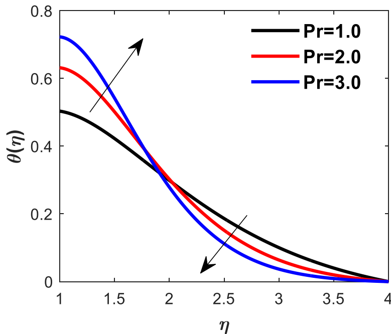
Figure 7: Effect of Prandtl's number on temperature
