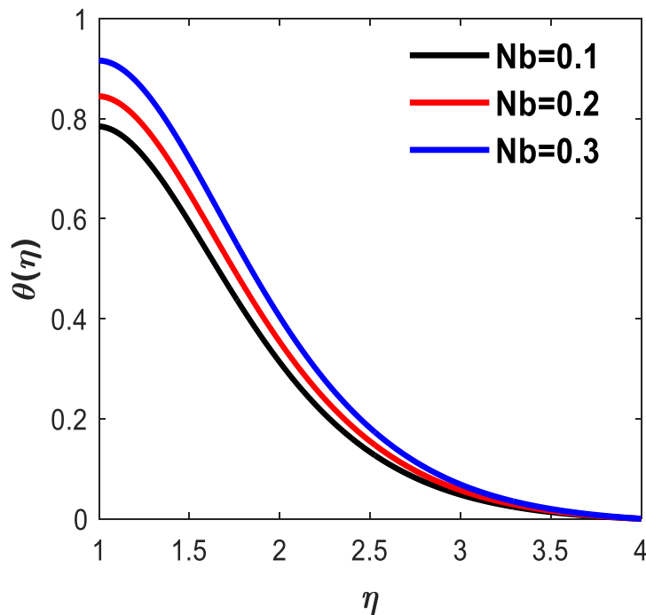
Figure 3: Effect of Brownian motion on temperature
