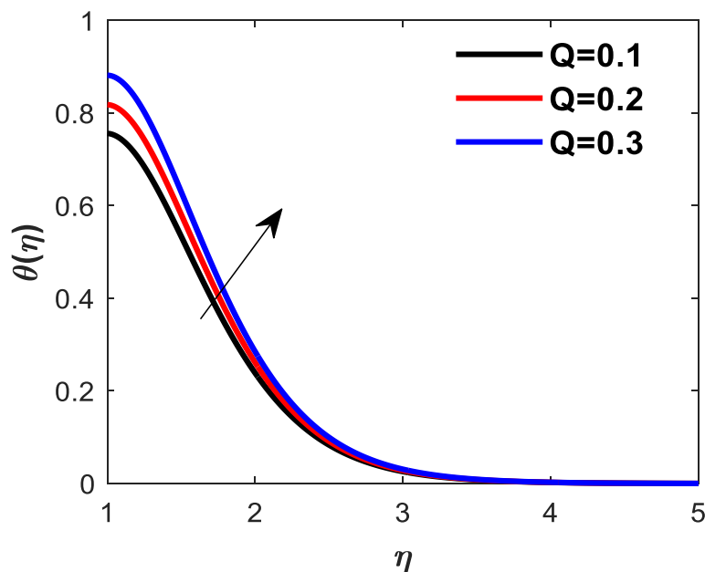
Figure 8: Effect of Joule heating parameter on temperature
