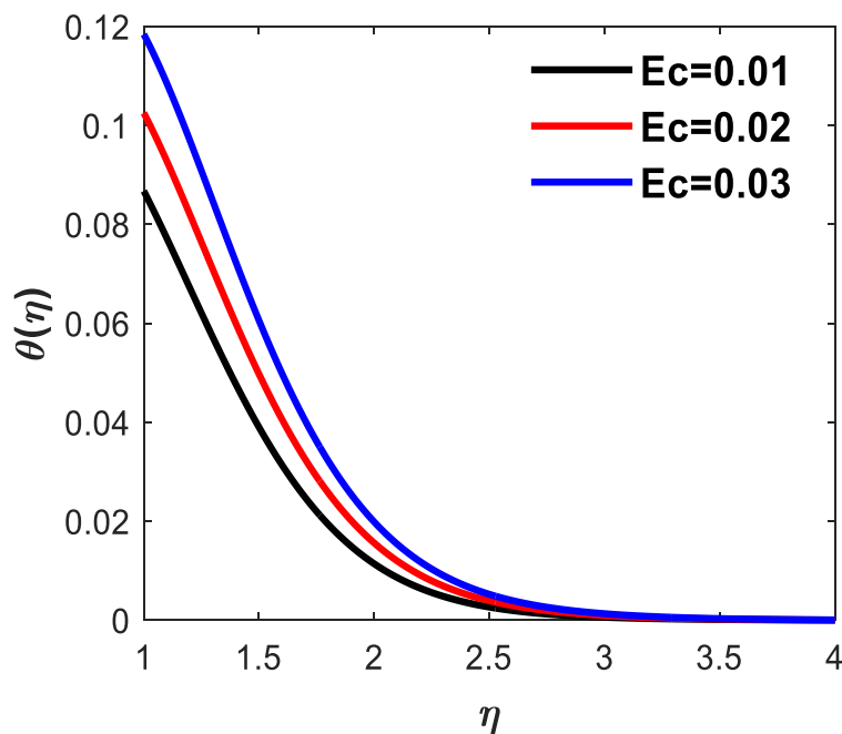
Figure 6: Effect of Eckert number on temperature
