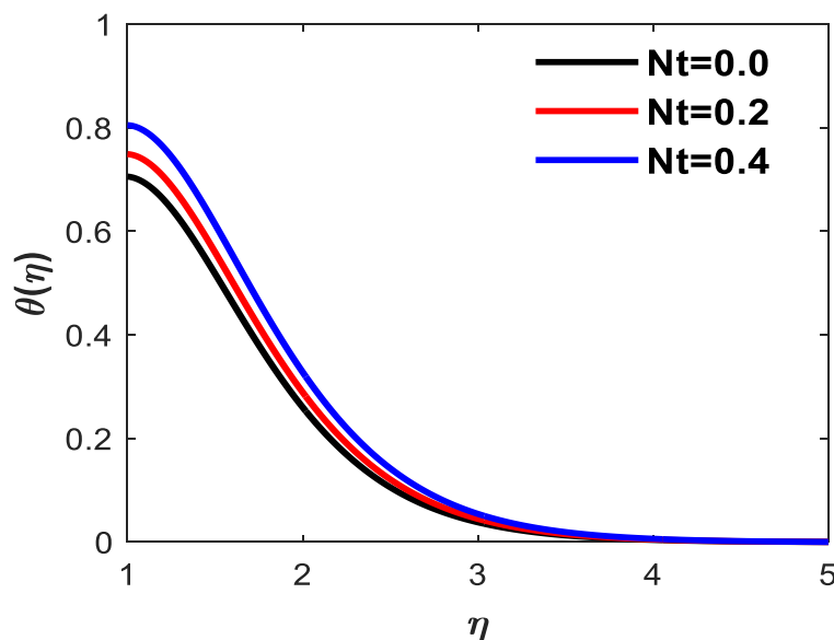
Figure 4: Effect of thermophoresis on temperature
