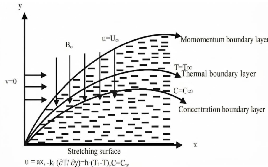
Figure 1: Geometry of the fluid flow
