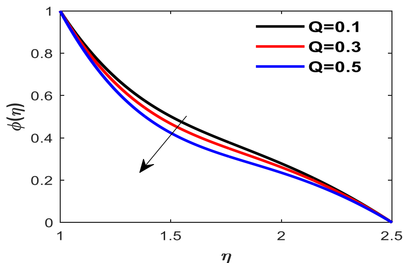
Figure 10: Effect of Joule heating parameter on concentration
